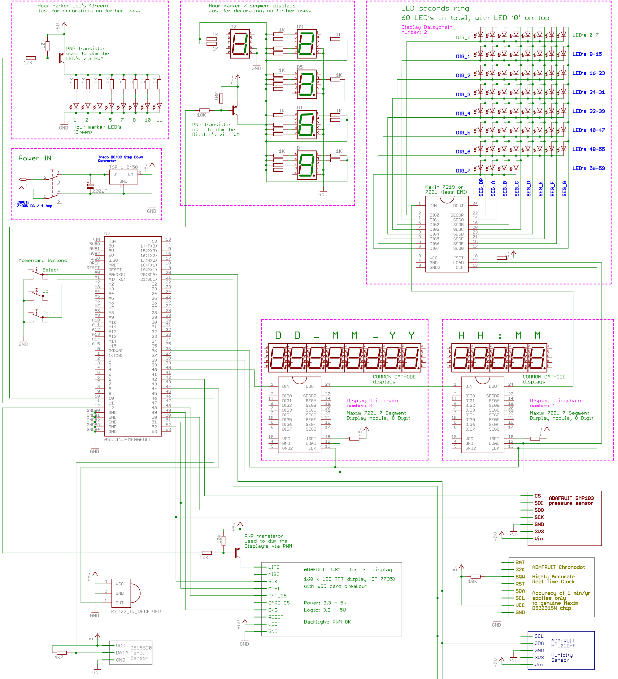
Gorgy Clock Schematic v1.0 2018-08-07
